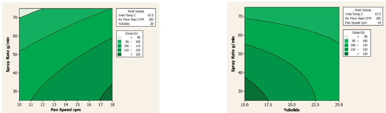
Figure 4. Contour Plots of Gloss versus Spray Rate, Pan Speed and % Solids
