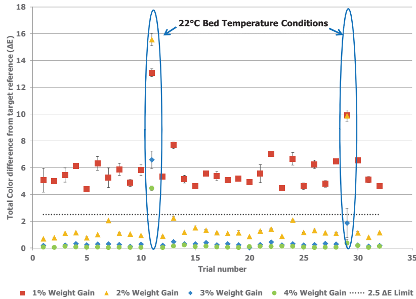
Figure 3. Color Difference from Target Reference \Delta E for Each Trial
