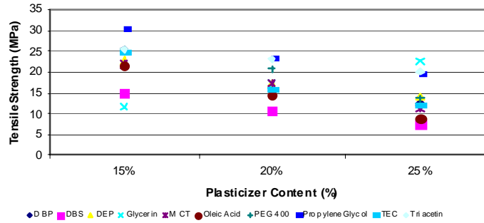
Figure 2. Plasticized Ethylcellulose Films: Tensile Strength Tensile Strength (MPa) versus Plasticizer Concentration
