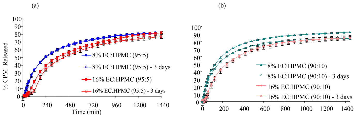
Figure 5. Dissolution Profiles of CPM Beads Coated with (a) EC:HPMC (95:5) and (b) EC:HPMC (90:10)
