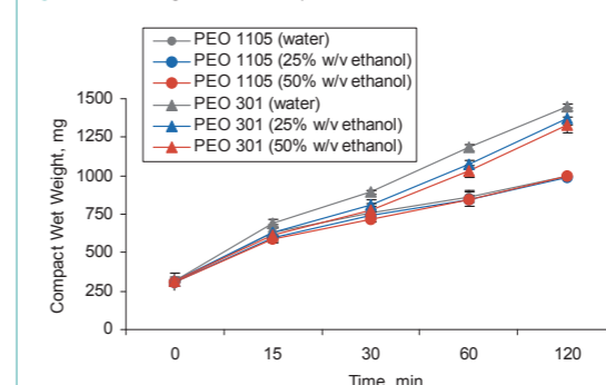
Figure 4. Wet Weight of PEO Compacts in Different Dissolution Media
