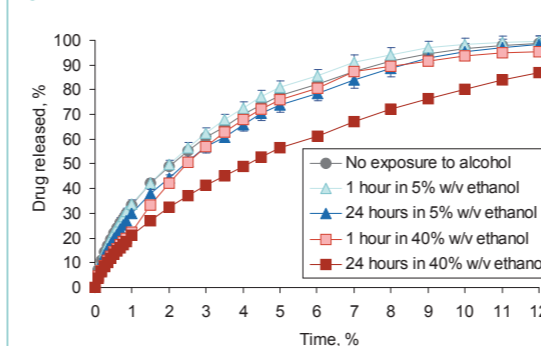
Figure 2. Metformin HCl Release in Different Dissolution Media
