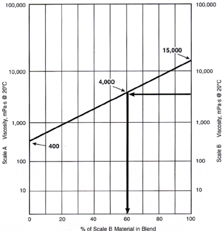
Figure 1. Blending Chart
