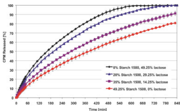
Figure 5. Effect of Starch 1500 levels on chlorpheniramine release from HPMC matrices manufactured at 14 kN. [Color figure can be seen in the online version of this article, available on the website, www.interscience.wiley.com .]
