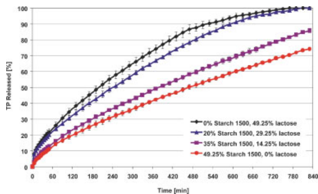
Figure 6. Effect of Starch 1500 levels on theophylline release from HPMC matrices manufactured at 14 kN. [Color figure can be seen in the online version of this article, available on the website, www.interscience.wiley.com .]
