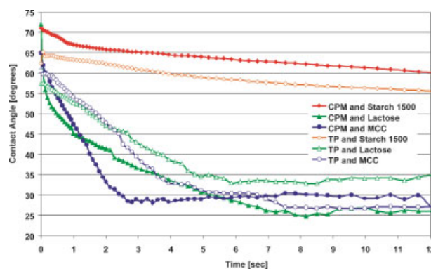
Figure 8. Contact angle measurements for water droplets on the surface of HPMC matrices containing different fillers. [Color figure can be seen in the online version of this article, available on the website, www.interscience.wiley.com .]
