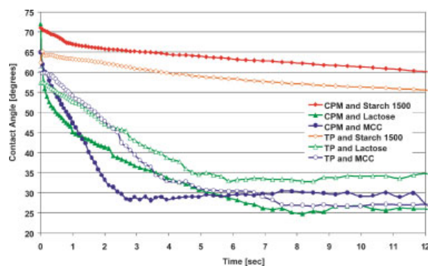
Figure 8. Contact angle measurements for water droplets on the surface of HPMC matrices containing different fillers. [Color figure can be seen in the online version of this article, available on the website, www.interscience.wiley.com .]
